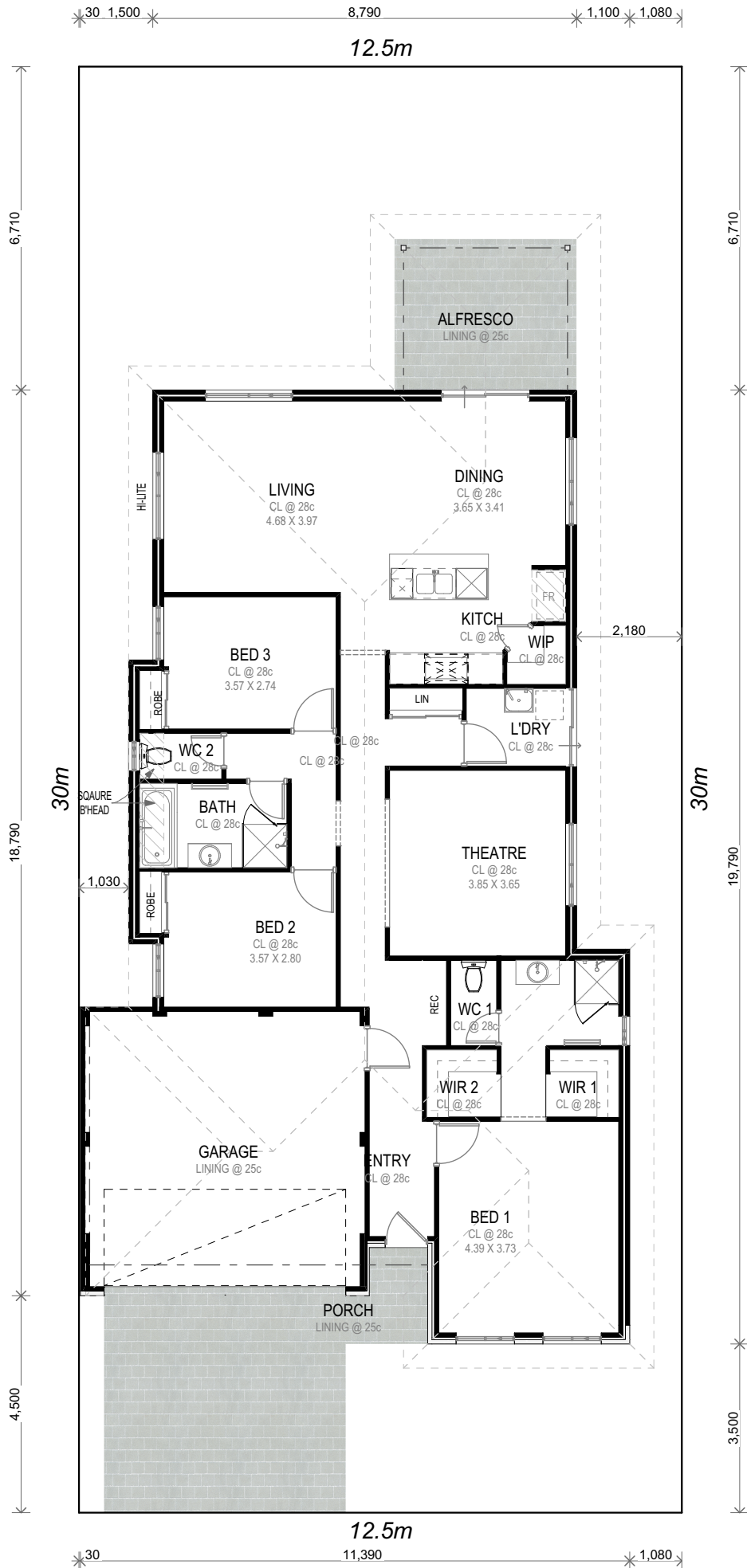
FLOOR PLAN NTS (FOR ILLUSTRATION PURPOSES ONLY)
